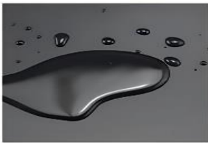
Residual sewage
